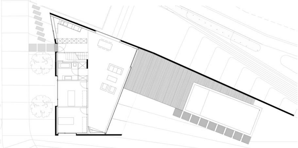
PLAN REZ
