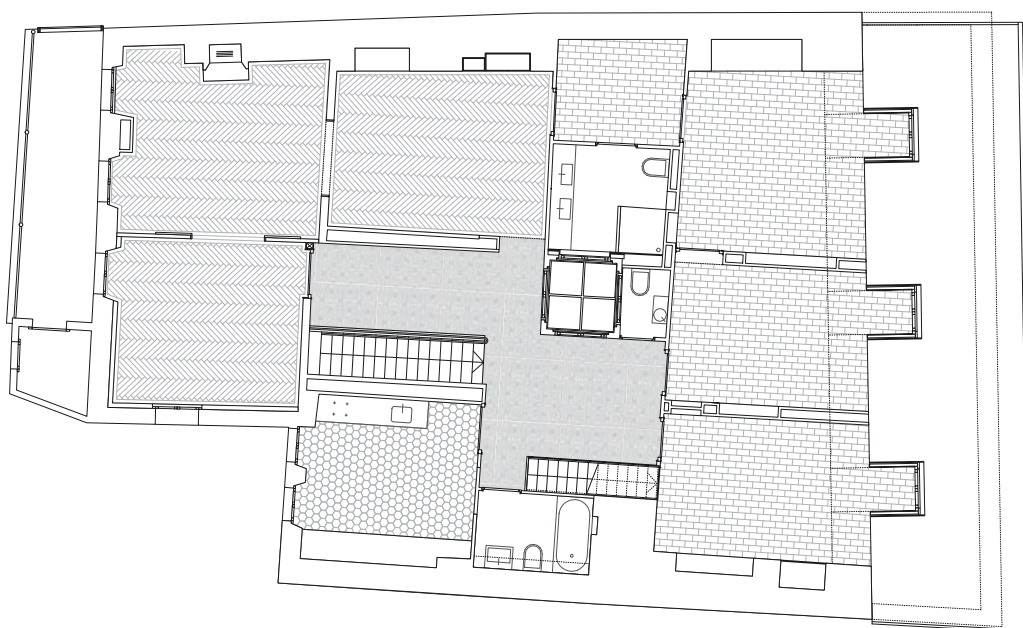
plan combles
