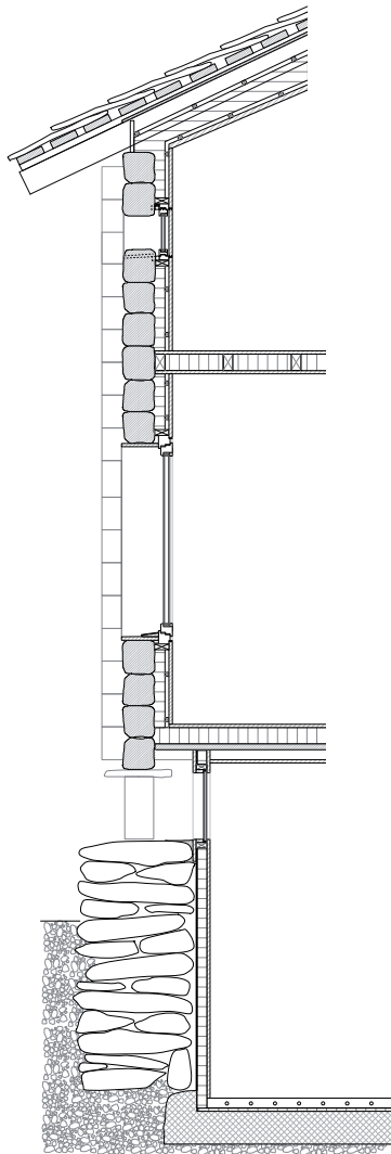
coupe constructive
