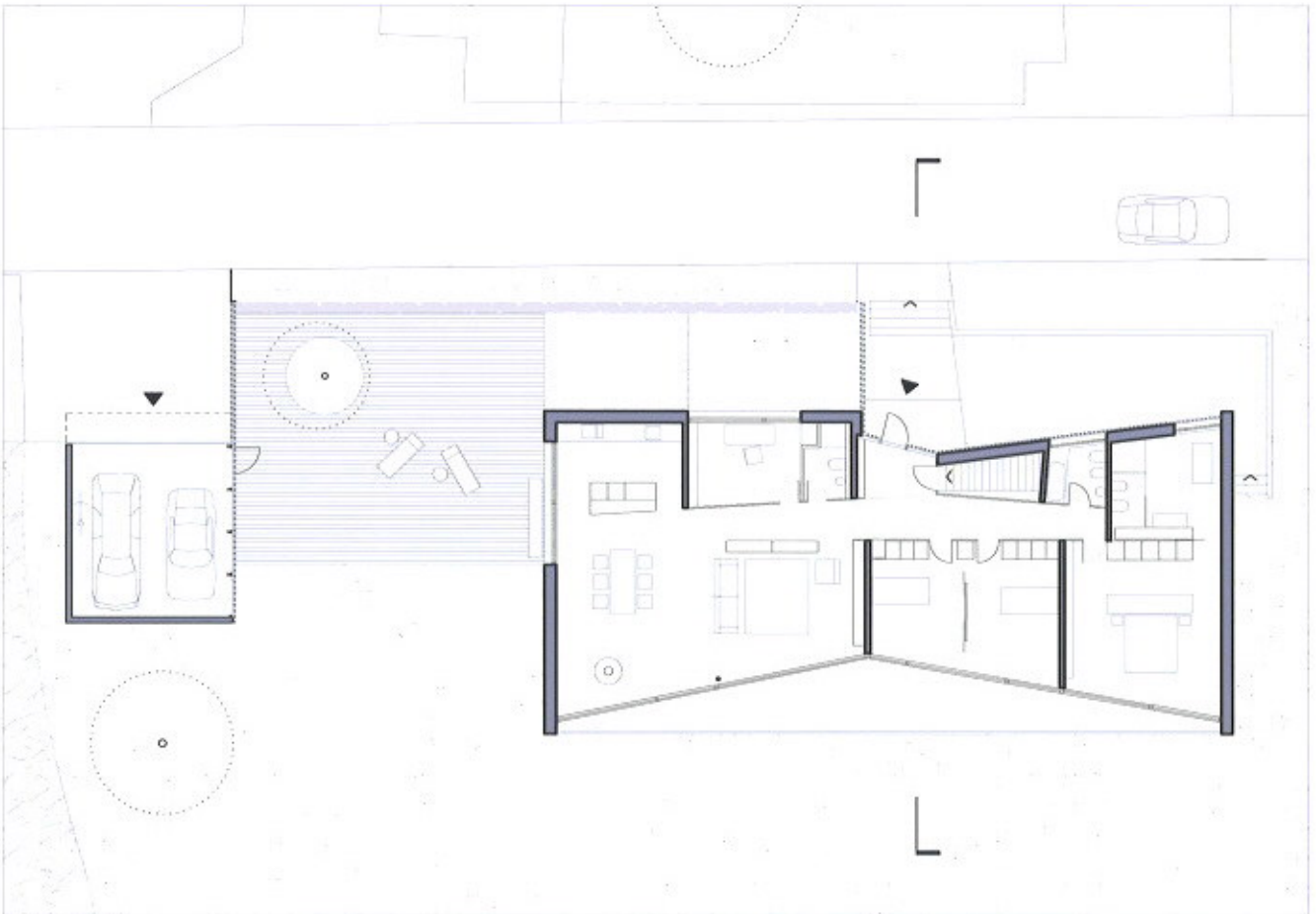
plan rez 1/250
